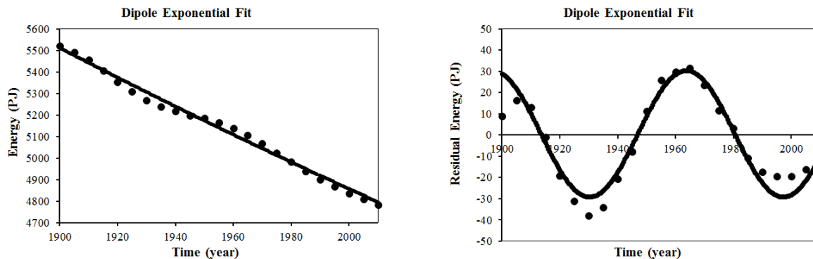
Figure 1. Dipole energy of the earth's magnetic field from 1900 to 2010 AD. The graph on the left shows the exponential fit. The graph on the right shows the sinusoidal fit to the residuals from the exponential fit.
