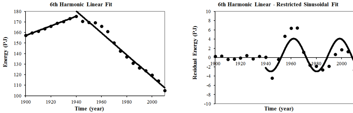
Figure 7. 6 th harmonic energy of the earth's magnetic field from 1900 to 2010 AD. The graph on the left uses two lines to fit the data. The graph on the right shows the sinusoidal fit to the residuals from the linear fit from 1940 to 2010 AD.
