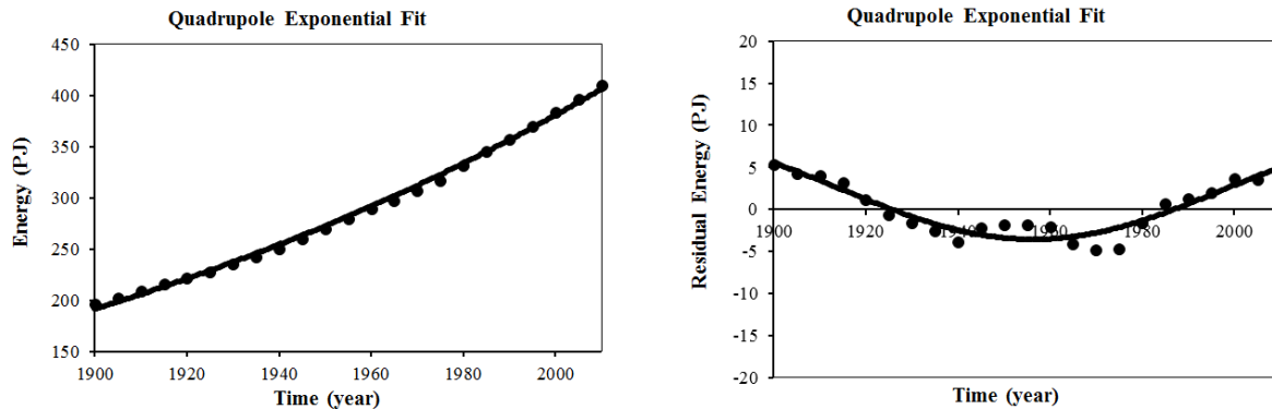
Figure 2. Quadrupole energy of the earth's magnetic field from 1900 to 2010 AD. The graph on the left shows the exponential fit. The graph on the right shows the sinusoidal fit to the residuals from the exponential fit.
