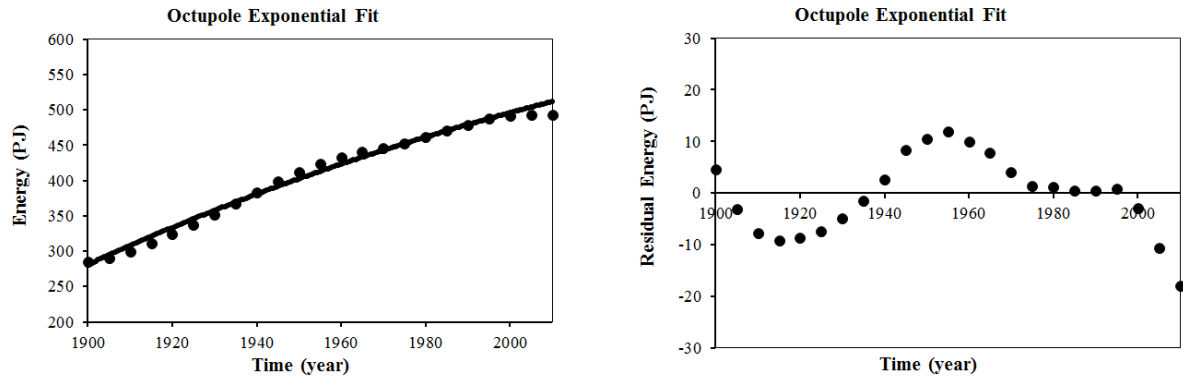
Figure 3. Octupole energy of the earth's magnetic field from 1900 to 2010 AD. The graph on the left shows the exponential fit. The graph on the right shows the sinusoidal fit to the residuals from the exponential fit. The sinusoidal fit was performed on data from 1900 to 1990 AD.
