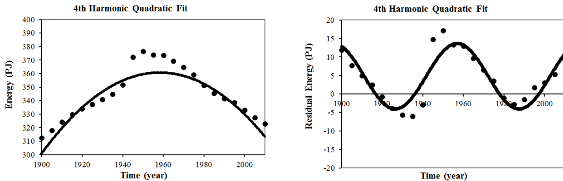
Figure 4. 4 th harmonic energy of the earth's magnetic field from 1900 to 2010 AD. The graph on the left shows the quadratic fit. The graph on the right shows the sinusoidal fit to the residuals from the quadratic fit.
