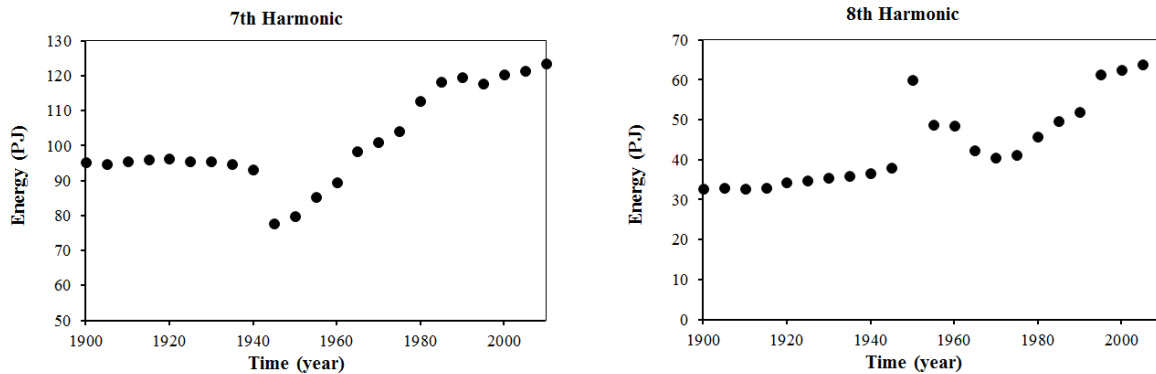
Figure 8. Higher harmonics of the earth's magnetic field from 1900 to 2010 AD. The graph on the left is the 7 th harmonic energy. The graph on the right is the 8 th harmonic energy.
