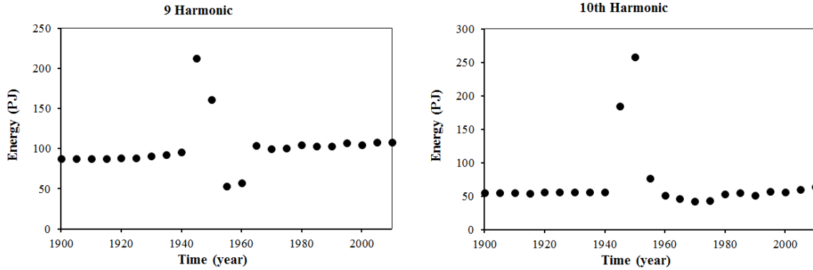
Figure 9. Higher harmonics of the earth's magnetic field from 1900 to 2010 AD. The graph on the left is the 9 th harmonic energy. The graph on the right is the 10 th harmonic energy.
