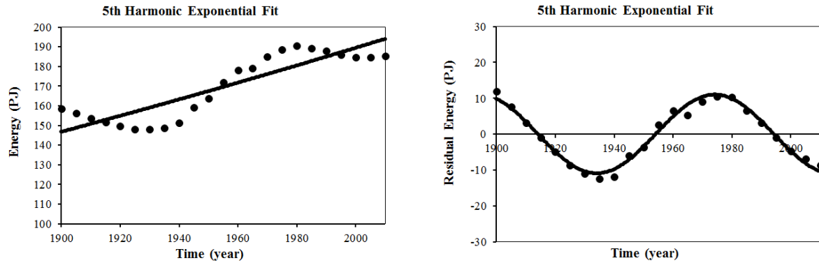
Figure 5. 5 th harmonic energy of the earth's magnetic field from 1900 to 2010 AD. The graph on the left shows the exponential fit. The graph on the right shows the sinusoidal fit to the residuals from the exponential fit.
