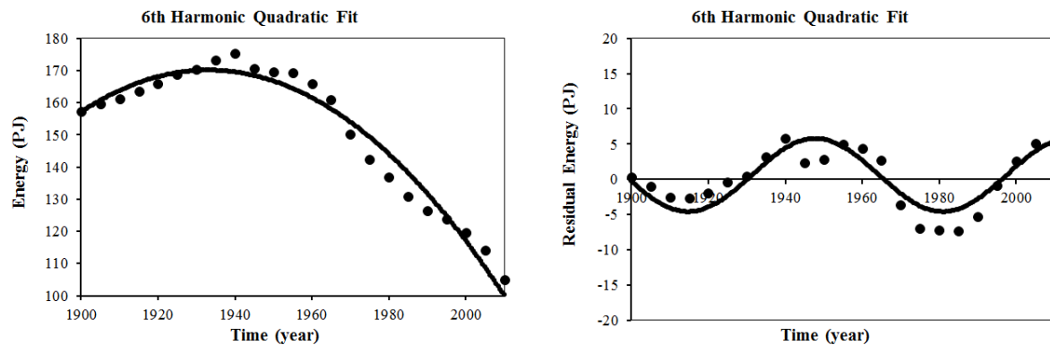
Figure 6. 6 th harmonic energy of the earth's magnetic field from 1900 to 2010 AD. The graph on the left shows the quadratic fit. The graph on the right shows the sinusoidal fit to the residuals from the quadratic fit.
