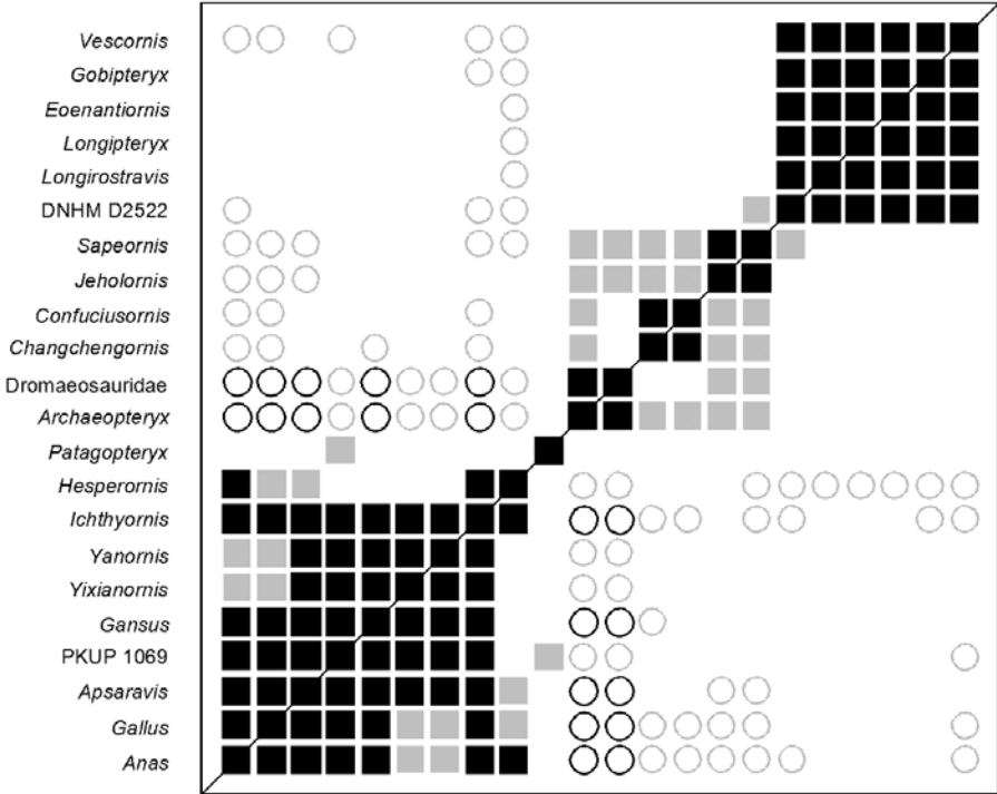
Figure 7. BDC results for O'Connor et al. 's (2009) matrix, as calculated by BDISTMDS (relevance cutoff 0.75). Closed squares indicate significant, positive BDC; open circles
