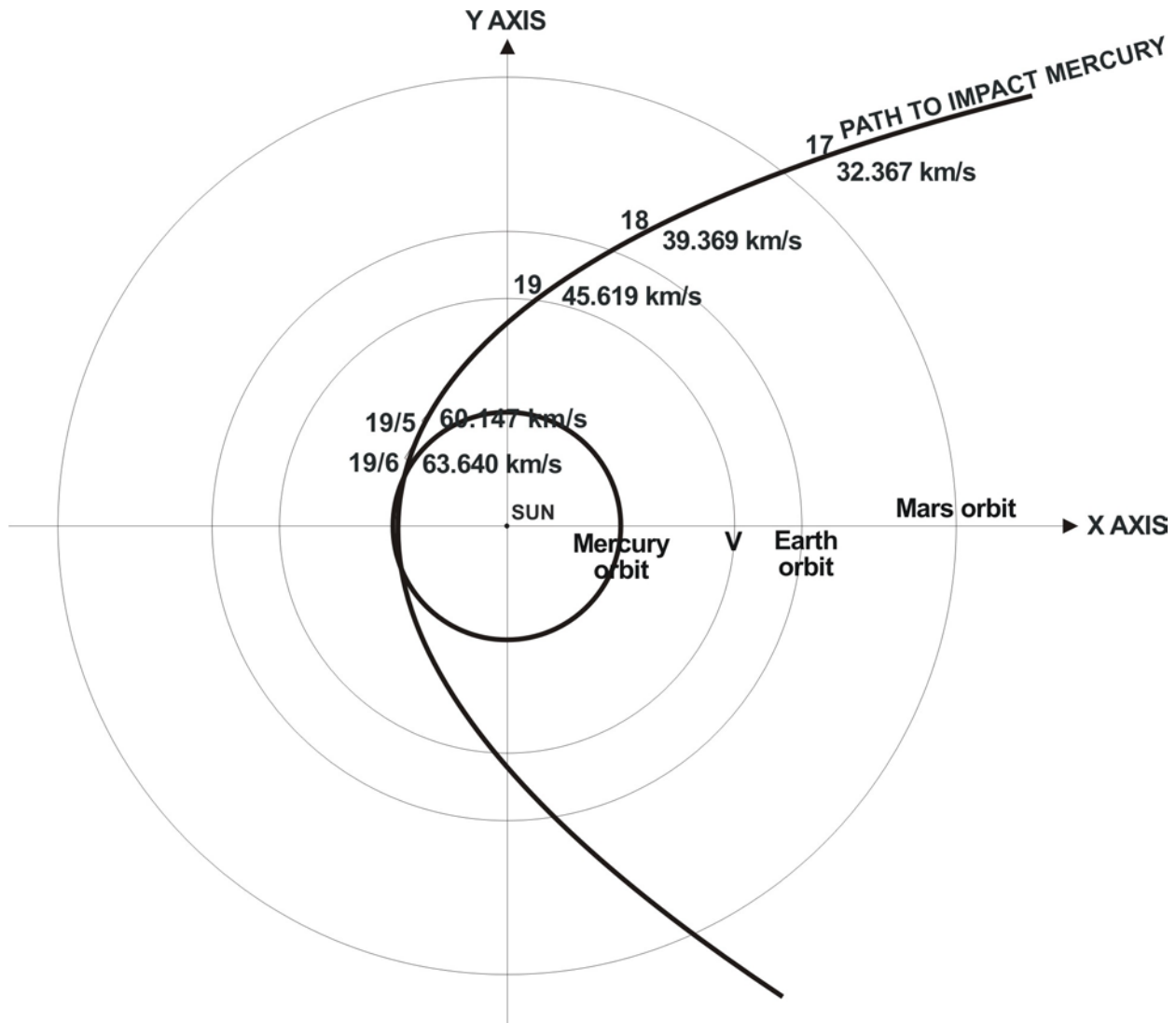
Figure 17. Impact with Mercury.
