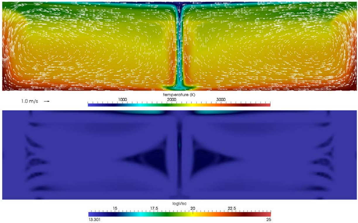
Figure 6. Day 45 after the onset of runaway for Case 1. The cold blob has reached the bottom of the mantle and the hot blob has risen into the upper mantle.
