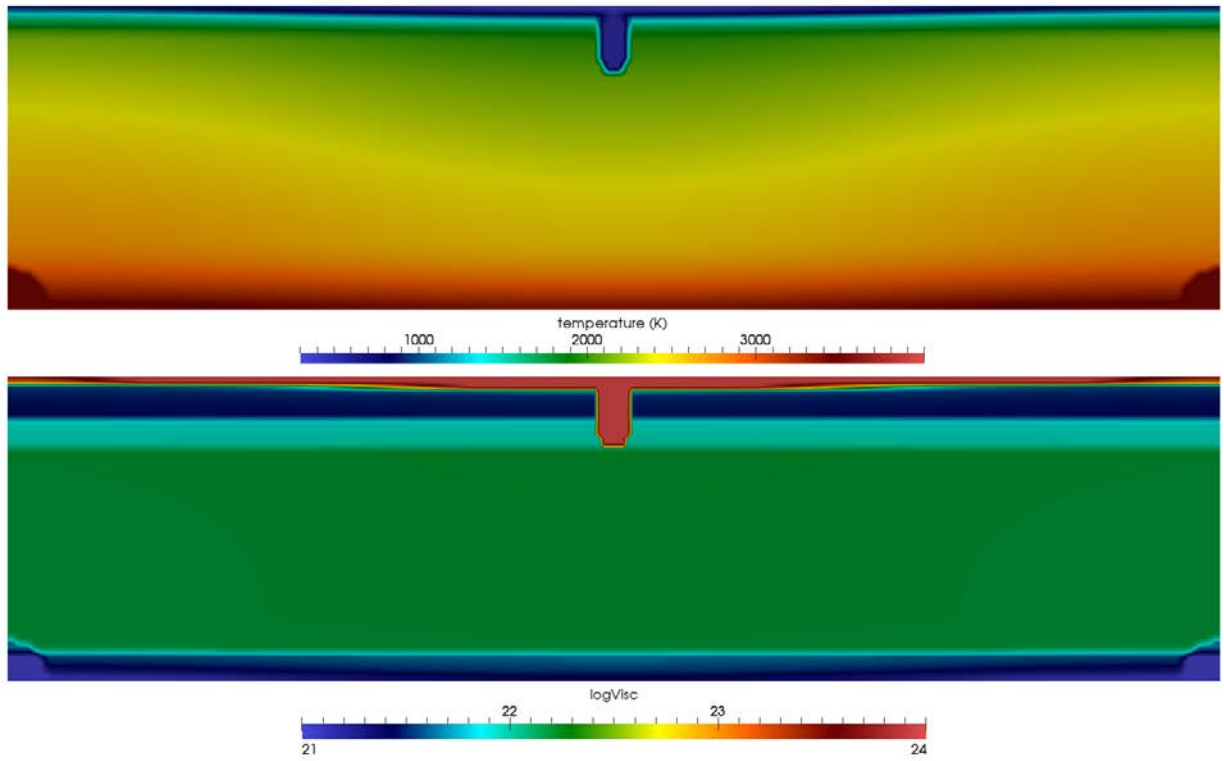
Figure 3. The initial temperature and viscosity fields for the Case 1 simulation with large initial temperature perturbations.
