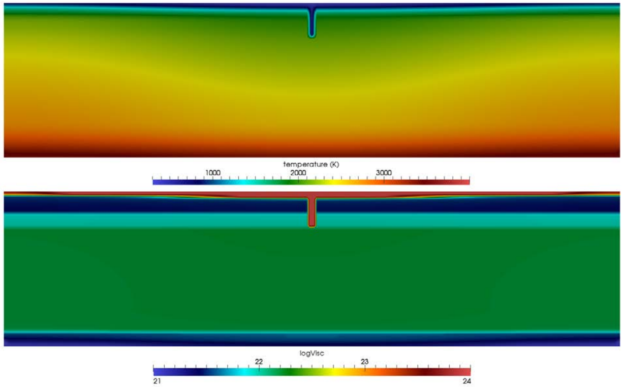
Figure 4. Initial viscosity and temperature fields for Case 2 with smaller initial temperature perturbations.
