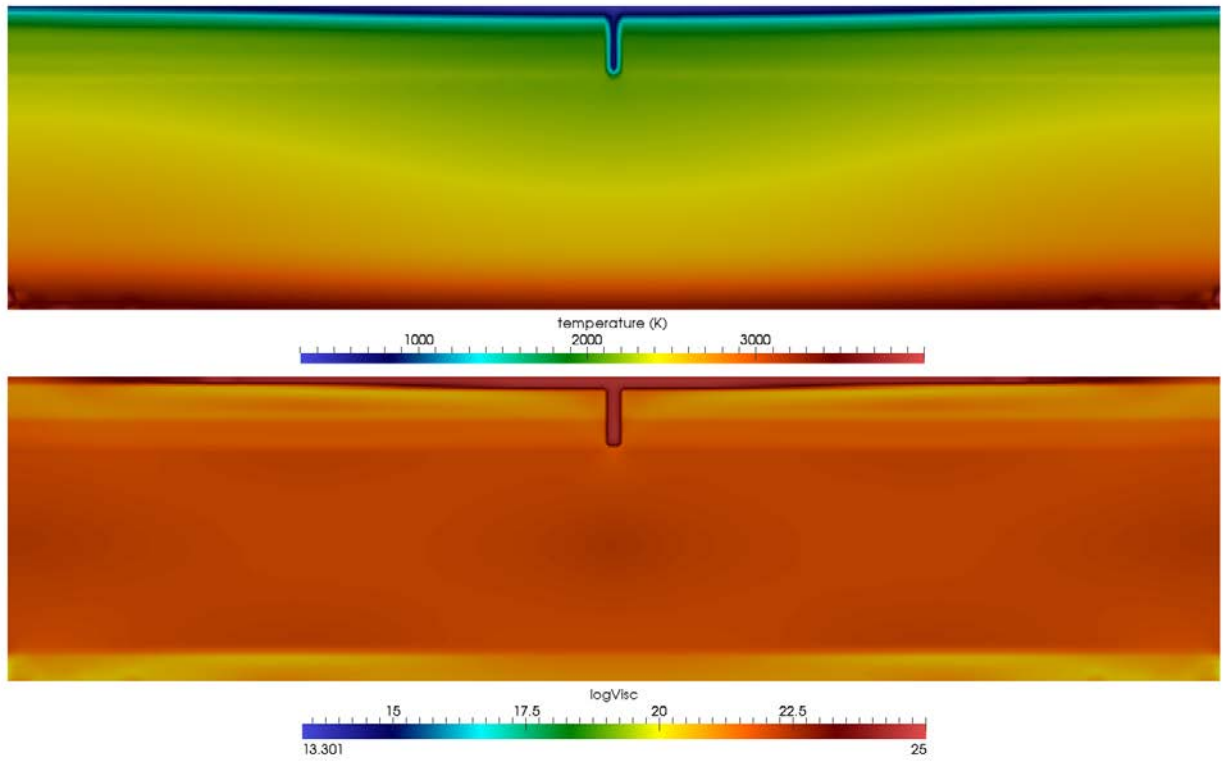
Figure 9. The temperature snapshot after 1.25 million years of simulation time for Case 2. The cold blob does not have enough gravitational potential energy to run away. Notice the viscosity distribution remains in the range of present day estimates.
