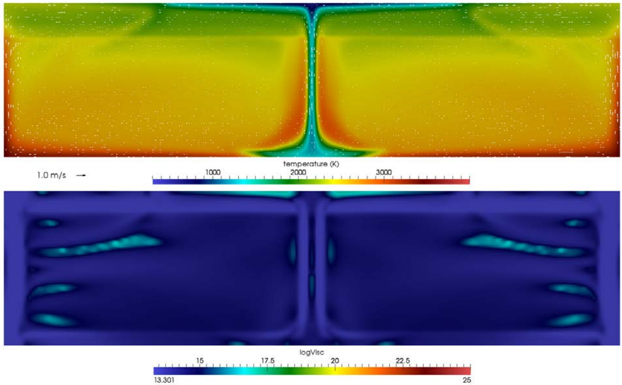
Figure 7. Day 80 after the onset of runaway for Case 1. The cold upper boundary layer continues to flow downward into the mantle. It is pushed laterally by the hotter material that has risen from below. Also notice the lower mantle is beginning to increase in strength in the areas away from the active upward and downward flow.
