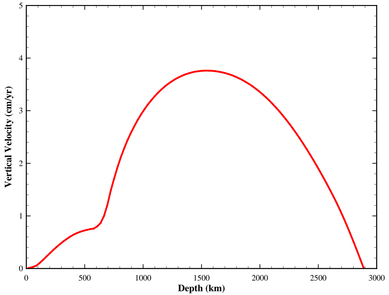
Figure 10. The vertical velocity profile through the thickness of the mantle for Case 2 at 1.25 million years simulation time.
