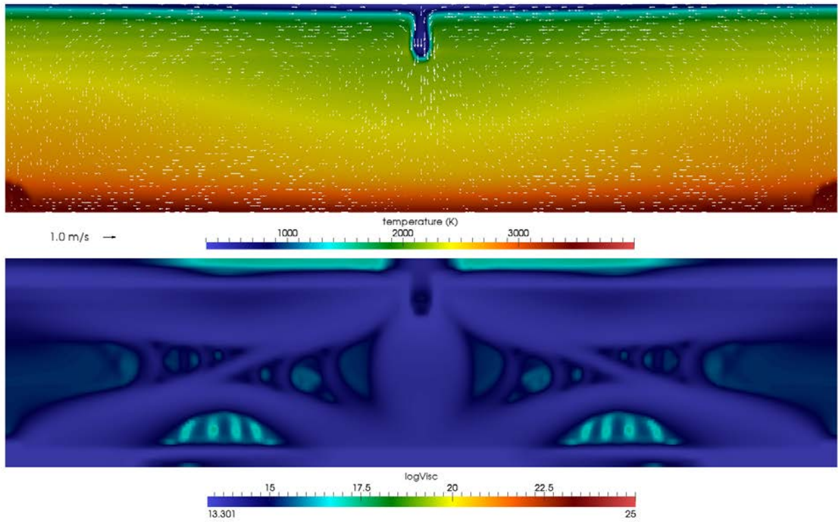
Figure 5. Day 2 after the onset of runaway for Case 1. Notice the low viscosity band (LVB) formed diagonally across the lower mantle.
