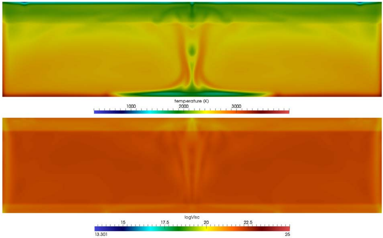
Figure 8. The end of the Case 1 simulation. The cold boundary layer has been completely transported to the bottom boundary, and the mantle has returned to near its original viscosity structure.
