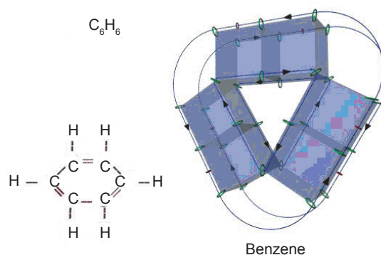
Figure 3. Benzene molecule. The cubes represent carbon atoms. The large rings are electrons and the small red rings are protons from the hydrogen atoms. Common edges reflect single bonds, common faces reflect double bonds, and blue lines represent magnetic flux lines that help bind the molecule together.
