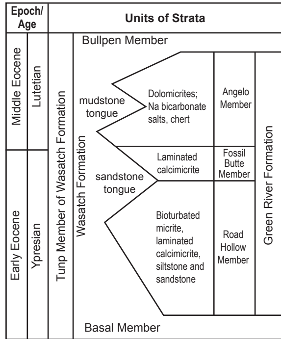
Figure 2. The Green River Formation often occurs as a lens of sediment within the Wasatch Formation, as shown here from Fossil Basin. Adapted and modified from Buchheim and Eugster (1998).
