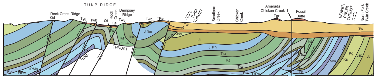
Figure 3. The Wasatch (Tw) and the Green River (Tgr) lie unconformably and nearly undeformed and horizontal on folded and thrustured Paleozoic and Mesozoic Rocks. The structural geology indicates the Laramide uplift and faulting which formed the Rocky Mountains must have occurred mostly before the sediments of the GRF were deposited, since they remain primarily undeformed. This cross section is representative of what lies below the Green River basins. Note the location of Fossil Butte which is near Kemmerer, Wyoming. Part of a west-east cross section (D-D') from Fossil Basin (Rubey, Oriol, & Tracey, 1975).
