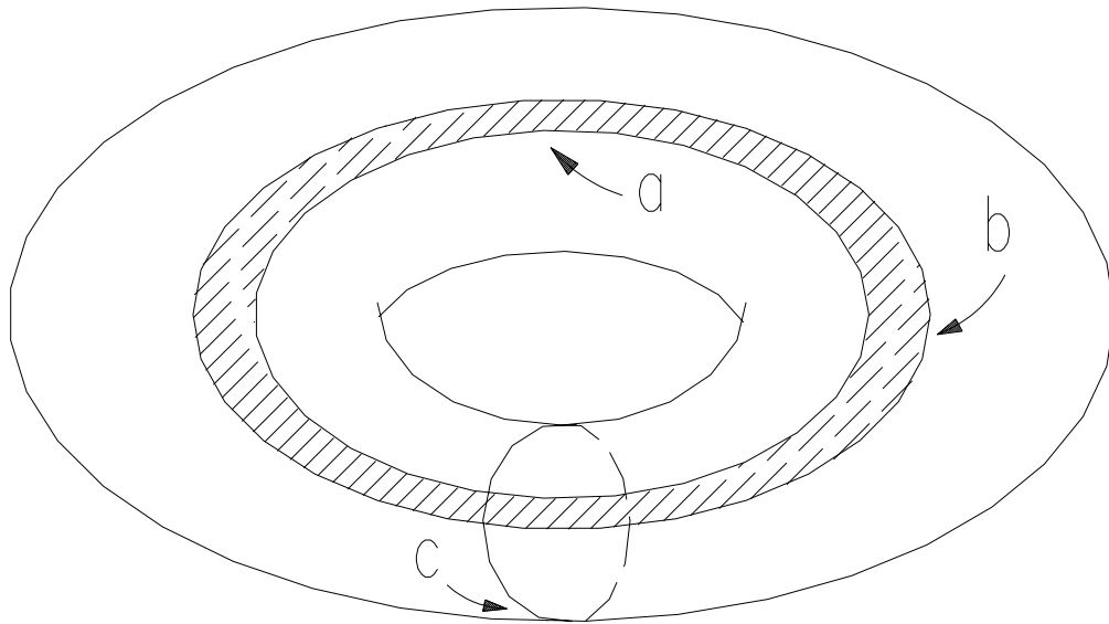
Figure 7. Three closed curves on the surface of a doughnut (torus) illustrate inequivalent and equivalent closed paths. Curves a and b , which bound the hatched area, can be smoothly distorted into each other, whereas curve c winds around a different direction and cannot be distorted into a or b , without cutting and pasting the ends (Figure drawn after Eguchi, Gilkey and Hanson, [20]).
