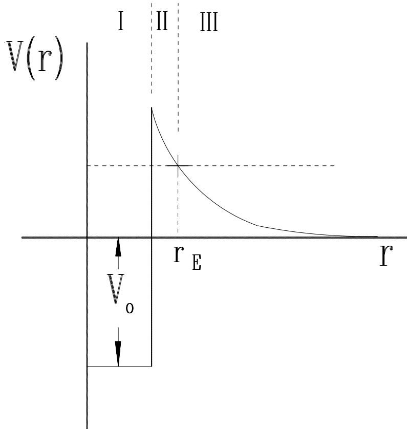
Figure 1. The Square-Well Potential with Coulomb Barrier
