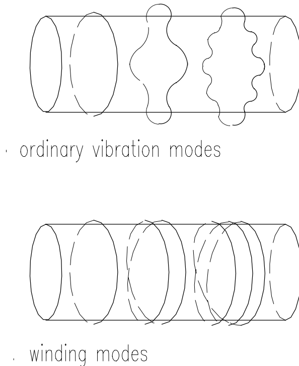
Figure 8. The ordinary vibration modes of closed strings (above) and the winding modes (below). In the equations of string theory, these two modes carry energy, and exchange roles when the radius of the compactified dimension moves from small to large.
