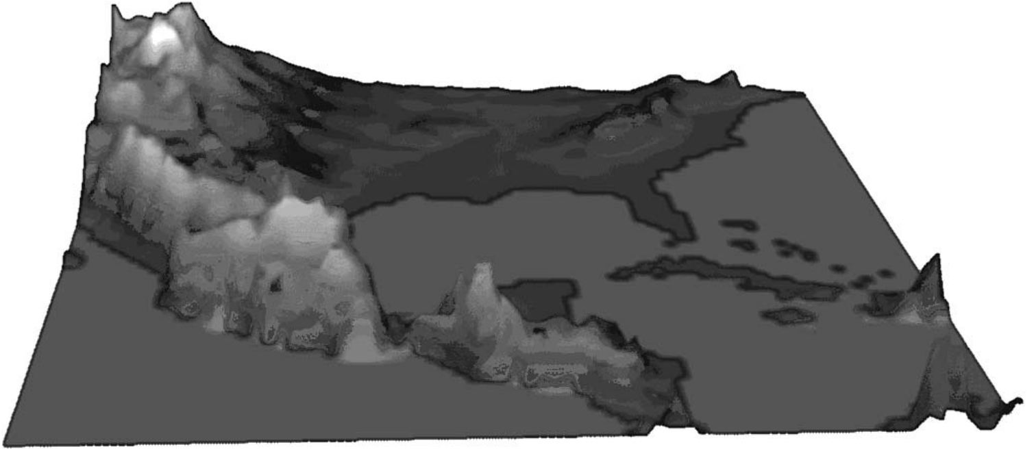
Figure 1. Perspective view of Hypercane Florence at 00Z on September 10, 1988 for a sea-surface temperature of 45°C. The cloud water content and precipitation water content did not exceed the display thresholds at this initial time.
