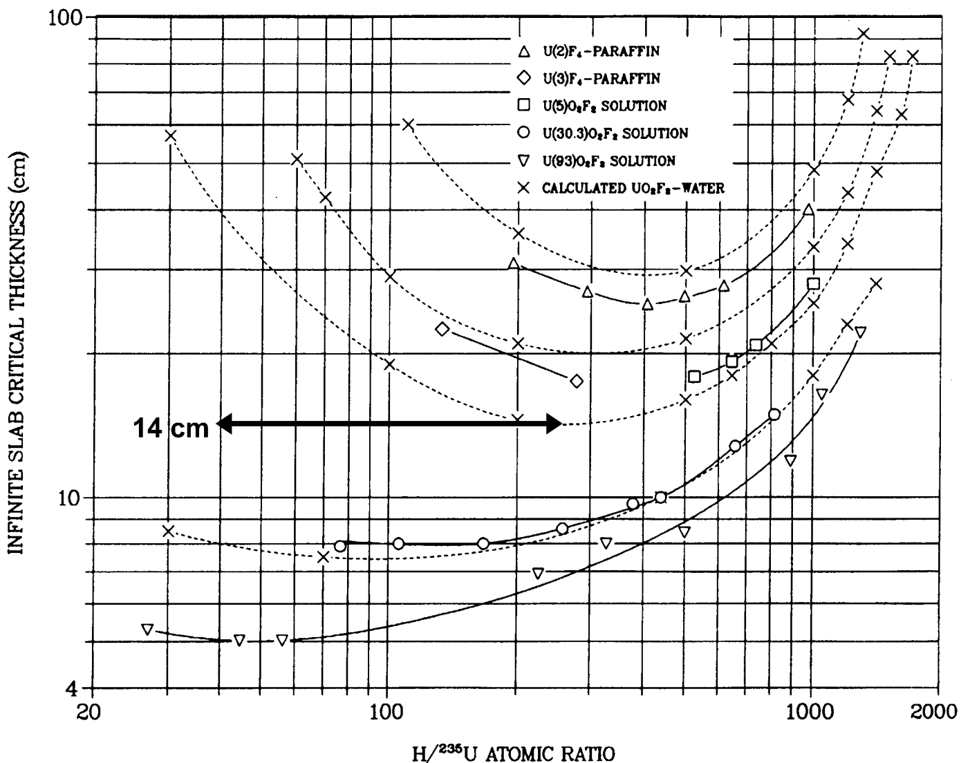
Estimated critical thicknesses of water-reflected slabs, infinite in other dimensions, of hydrogen-moderated U(93), U(30.3), U(5.00), U(3.00) and U(2.00).
