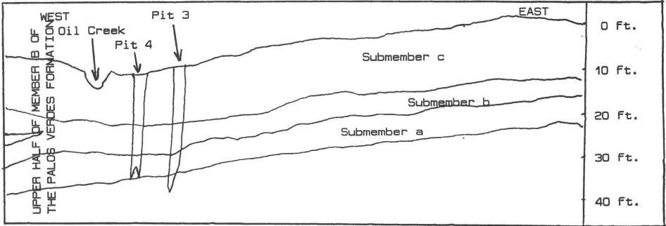
Figure 1. A cross section of the fossiliferous strata at Rancho La Brea, along an east-west direction across Hancock Park. From Shaw and Quinn (1986) [27, p.8].
