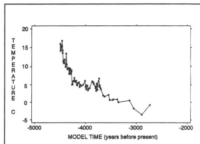
Figure 1 Cooling of polar bottom water after the Flood. From [107]. Data from [46,90].
