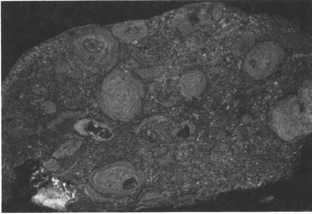
Figure 10. Algal coating around shell fragments in section known as Sphaerocodium . Occurrences in rocks of the Lower Palaeozoic indicate that the original sediments remained exposed on shallow platforms for some time after the Flood year. The above specimen is from the Upper Muschelkalk, Triassic, of Germany. Slightly enlarged.
