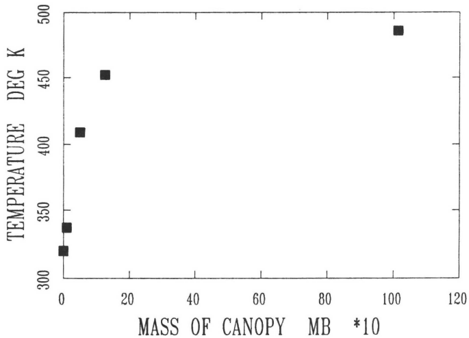
Fig. 4. Radiative equilibrium surface temperature as a function of mass of the overlying canopy.
