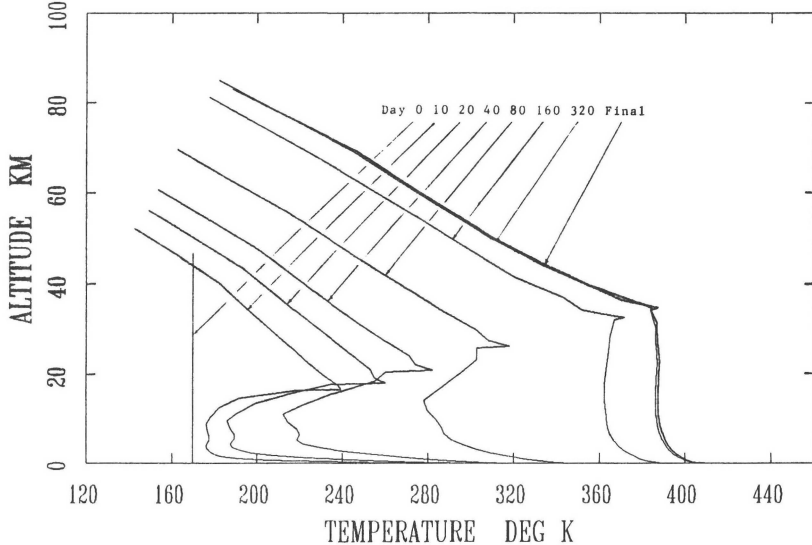
Fig. 2. Vertical temperature profiles of a 50mb canopy above today's atmosphere starting from an isothermal 170° condition approaching equilibrium.
