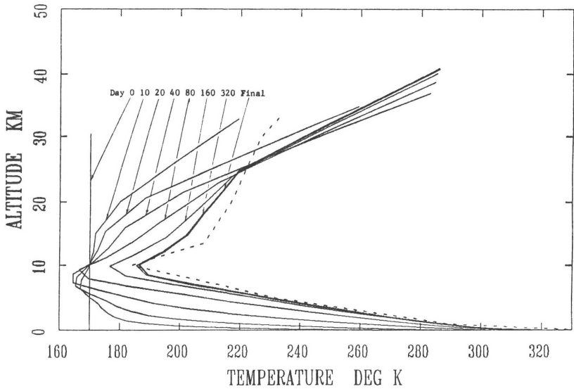
Fig. 1. Vertical temperature profile for today's atmosphere starting from an isothermal 170° condition approaching the Manabe and Strickler (1964) result. Solid profiles are model results at indicated days after day 0 and dashed line is MS profile.
