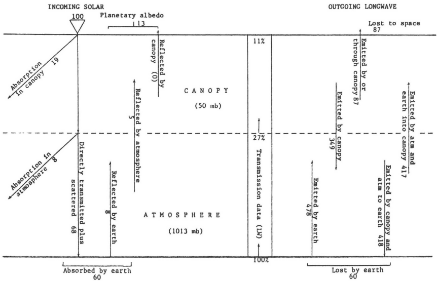
Fig. 3. The heat balance of the earth-atmosphere-canopy system for a 50mb canopy over today's atmosphere. The left portion of the diagram shows the flux of short-wave radiation, the right portion the flux of long-wave radiation, and the middle portion the transmission of long-wave radiation upward to space. The canopy is above the dashed line and the atmosphere is below the dashed line.
