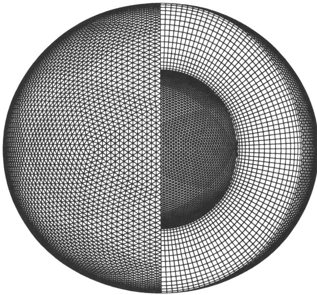
Figure 2. Cutaway view of the computational mesh for spherical shell used in 3-D finite element calculation. Mesh has seventeen layers of cells with 10242 cells in each layer.
