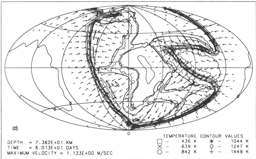
Figure 4. Snapshots from a 3-D calculation to investigate the consequences of initial subduction about a Pangean supercontinent. (a) Initial temperature contours and outlines of continental units that are treated as separate elastic/plastic blocks. (b)-(d) Solution after 20, 40, and 60 days, respectively, at a depth of 74 km. Finer lines are temperature contours, coarser lines are the 80% of initial continental thickness contour, and arrows represent the velocity field.
