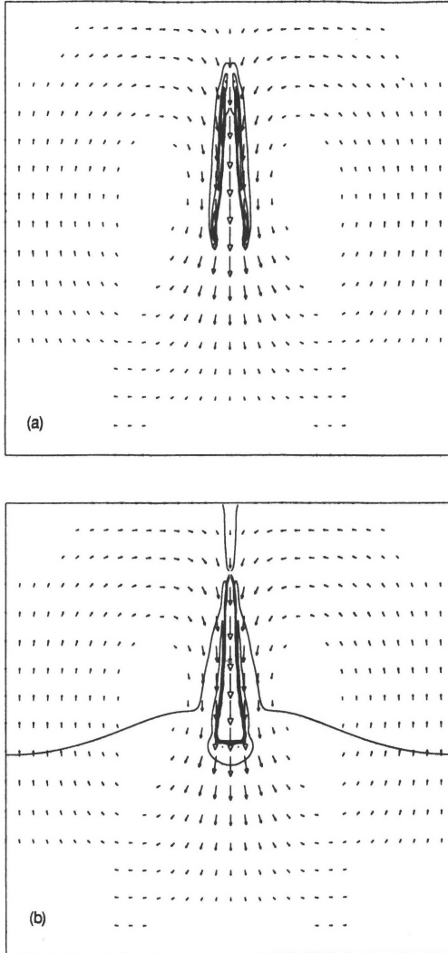
Figure 1. Snapshot from a calculation of the sinking of a vertical slab in a temperature--dependent viscous fluid just prior to thermal runaway. (a) Contours of shear heating rate show heating is strongly localized in zone next to slab. (b) Contours of the logarithm of viscosity show contour of minimum viscosity enclosing bottom of slab. Arrows denote the velocity field.
