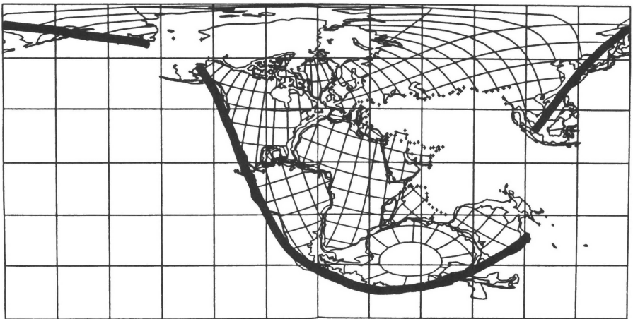
Figure 3. Reconstruction of Pangea published by Smith, Hurley, and Briden (8). The dark band indicates the distribution of initially subducting ocean lithosphere in the 3-D calculation.
