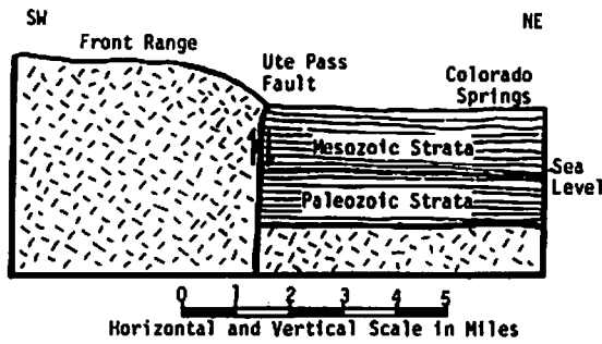
FIGURE 5. Cross section of Ute Pass Fault southwest of Colorado Springs, Colorado. Precambrian basement rocks have been uplifted many thousands of feet on the west side of the fault.
