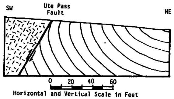
FIGURE 6. Cross section of Ute Pass Fault one mile southeast of Manitou Springs, Colorado. Pike's Peak granite on southwest side of fault has been upthrown thousands of feet to deform Fountain Formation, arkosic sandstone strata. The intensity of drag folding dies out dramatically within several tens of feet northeast of the fault.
