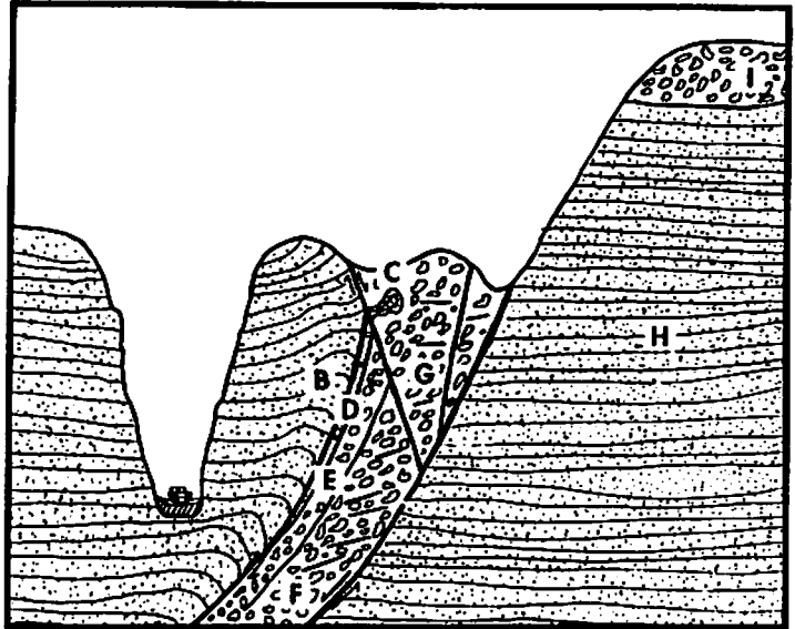
FIGURE 1. Cross section of the Split Mountain Fault drawn perpendicular to the plane of the fault. A large volume of sedimentary boulder breccia slipped down into the hole created by slip on the concave upward normal fault. Zones labeled by letter are explained below. Automobile in gorge provides scale.
