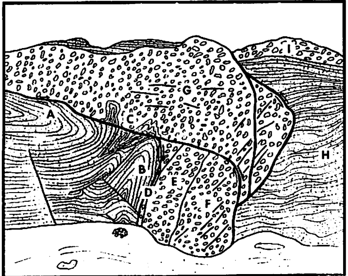
FIGURE 2. Overview from east side of Split Mountain Gorge of cliff and slope of the west side of the gorge showing numerous soft sediment deformation features associated with the fault. Zones labeled by letter are explained below. Automobile at base of cliff provides scale.
