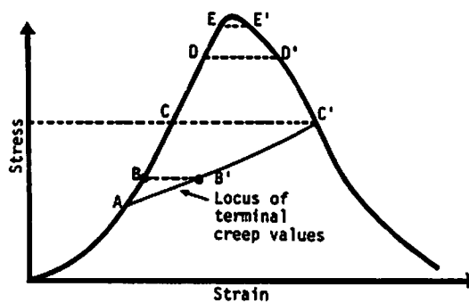
FIGURE 4. A complete stress-strain curve showing the limits of time-dependent strain on rock (after Goodnan 1980, p. 74).
