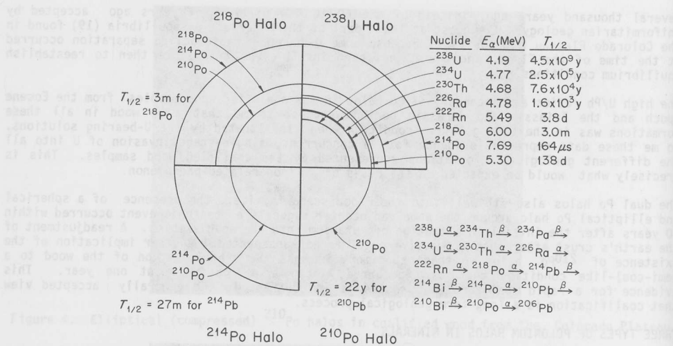
Figure 7. Idealized schematic of ^{238}\text{U} , ^{218}\text{Po} , ^{214}\text{Po} , and ^{210}\text{Po} halos.
