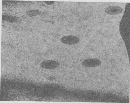
Figure 4. Elliptical (compressed) ^{210}\text{Po} halos in coalified wood from the Colorado Plateau.
