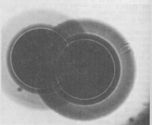
Figure 11. ^{218}\text{Po} halo in mica.
