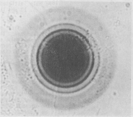
Figure 10. ^{238}\text{U} in mica.
