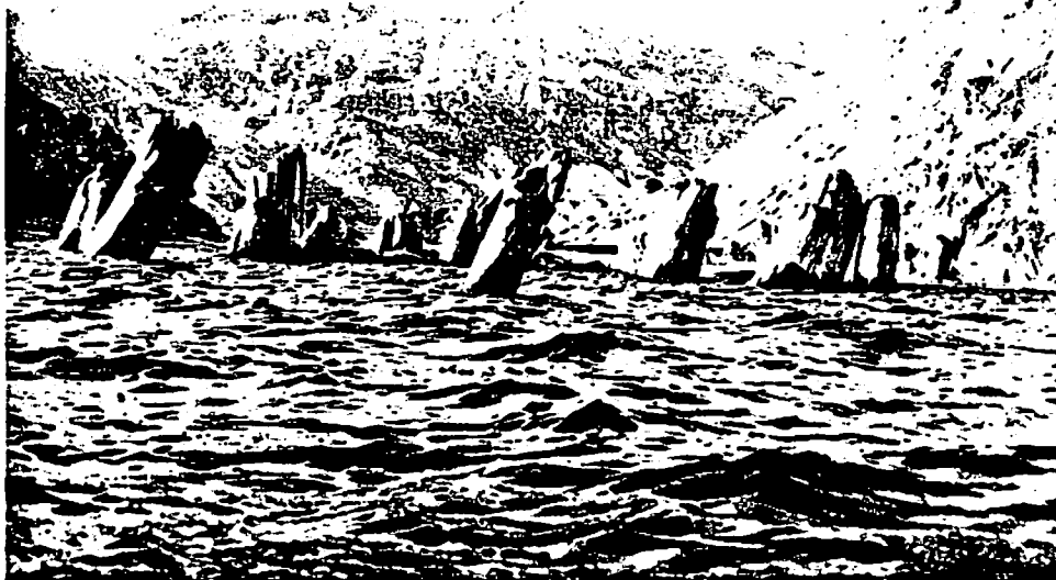
FIGURE 6. Upright trunks of trees deposited on the north shore of Spirit Lake. The trunks are slightly inclined due to manmade lowering of the level of the lake.
